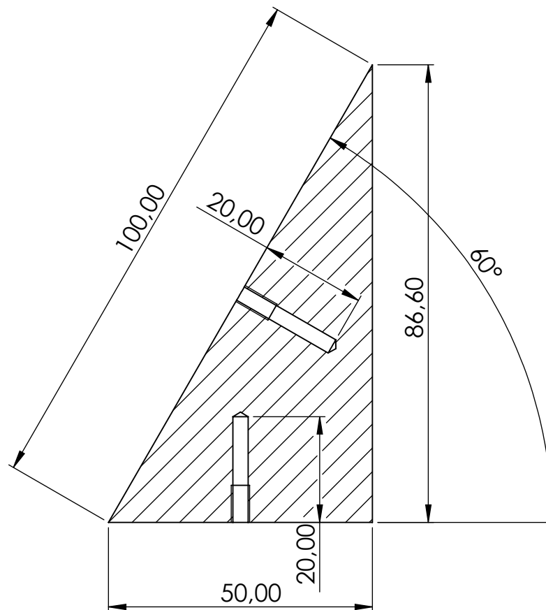
SECTION C-C
